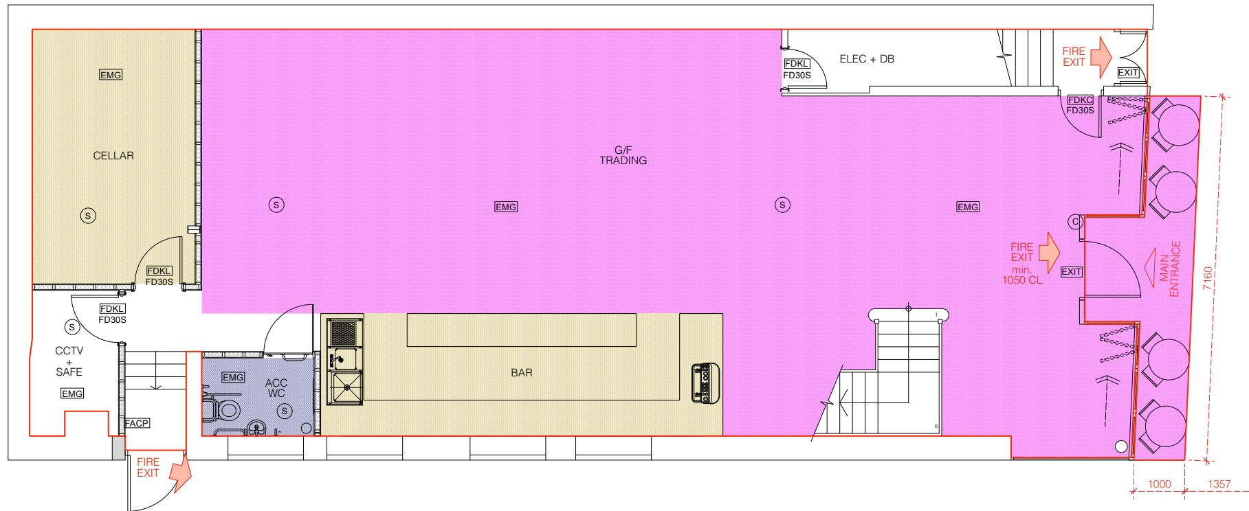
PROPOSED GROUND FLOOR PLAN Scale 1:50@A1, 1:100@A3
