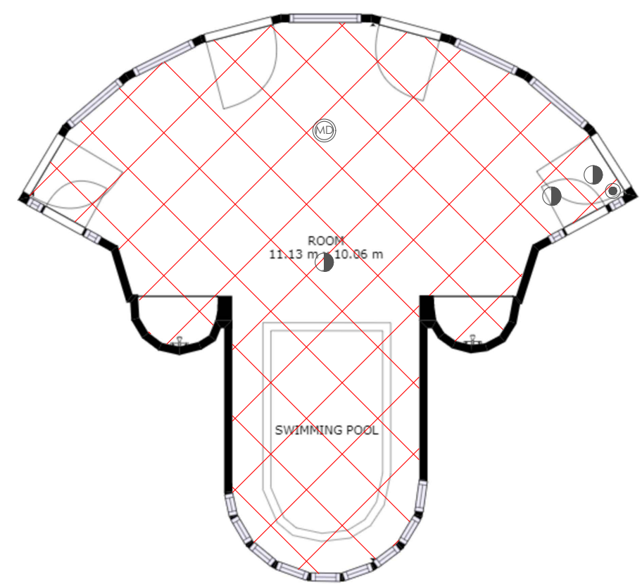
GROUND FLOOR AND SPA BUILDING
