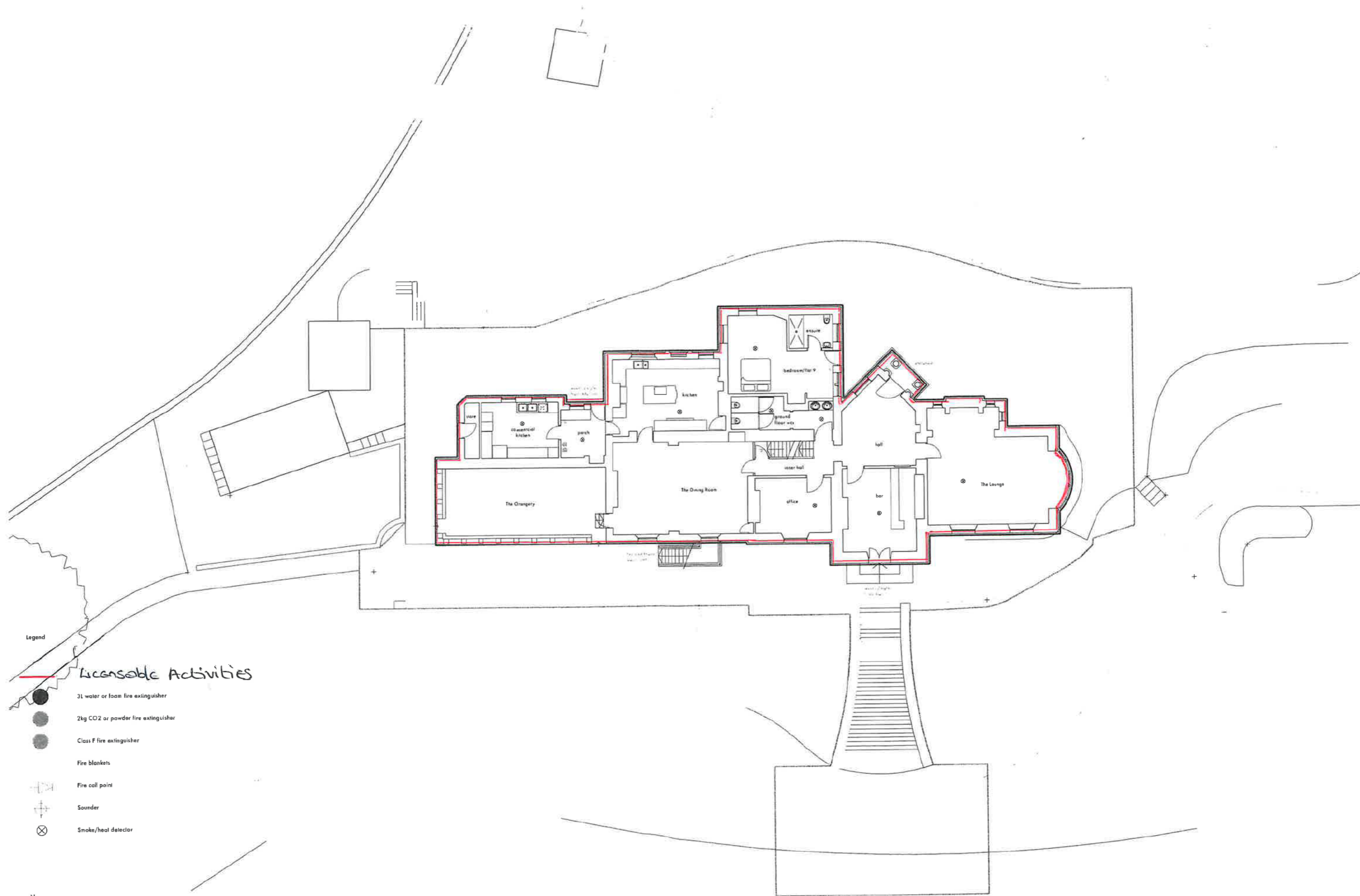
Carke Manor - Ground Floor Plan
